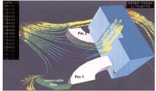
Option 2 - Removable shutters and guide fins
