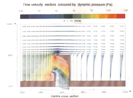
Flow velocity vectors
