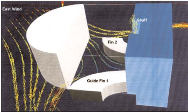
Base air flow CFD with options
