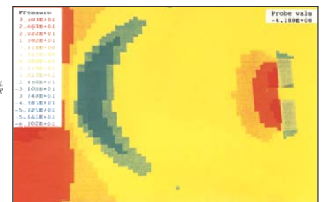
CFD of wind pressure over rooftop
