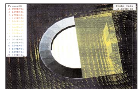
CFD of East Wind over rooftop
