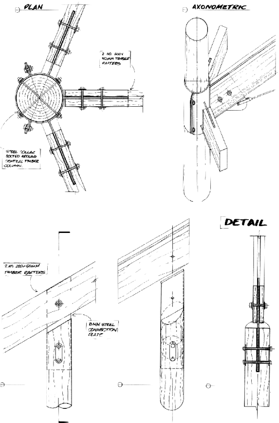
Structural details
